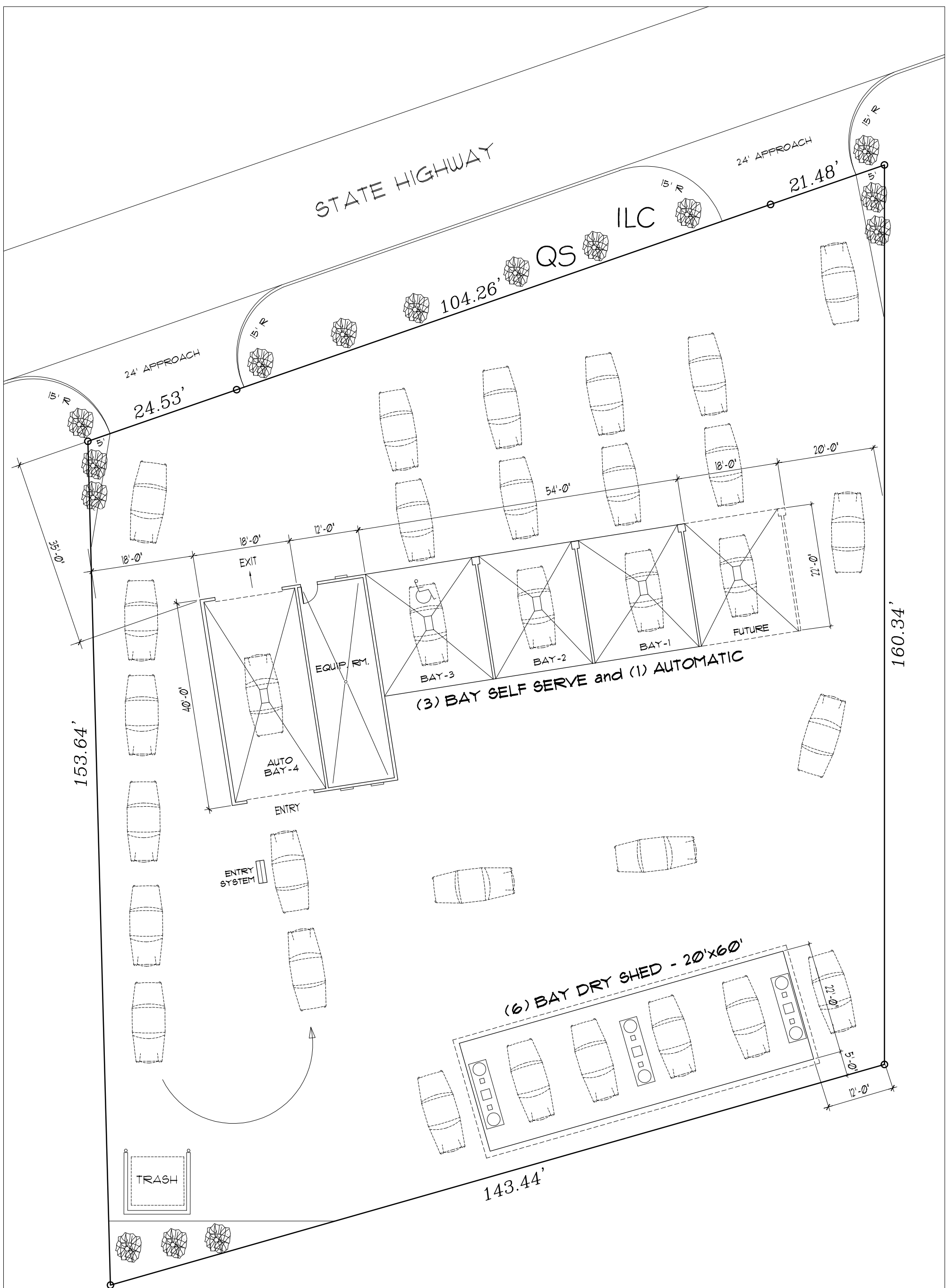
SITE PLAN - L
