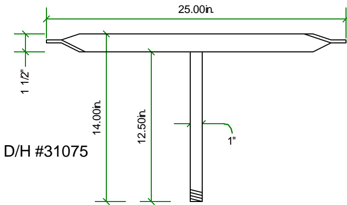
STANDARD DOUBLE BOOM
