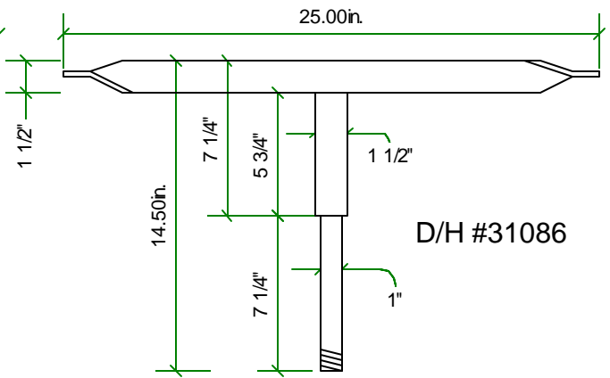
EXTENDED SINGLE BOOM
