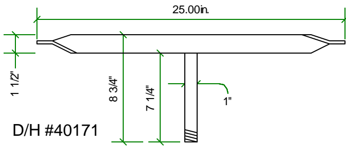
STANDARD SINGLE BOOM
