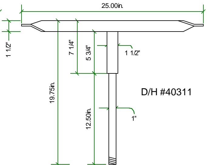
EXTENDED DOUBLE BOOM
